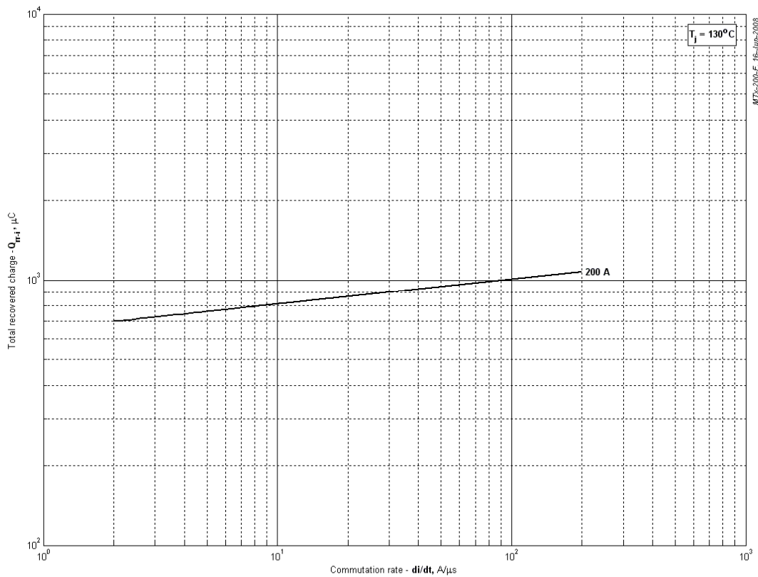
Fig 5 - Total recovered charge, Q_{tr-i} (integral)
