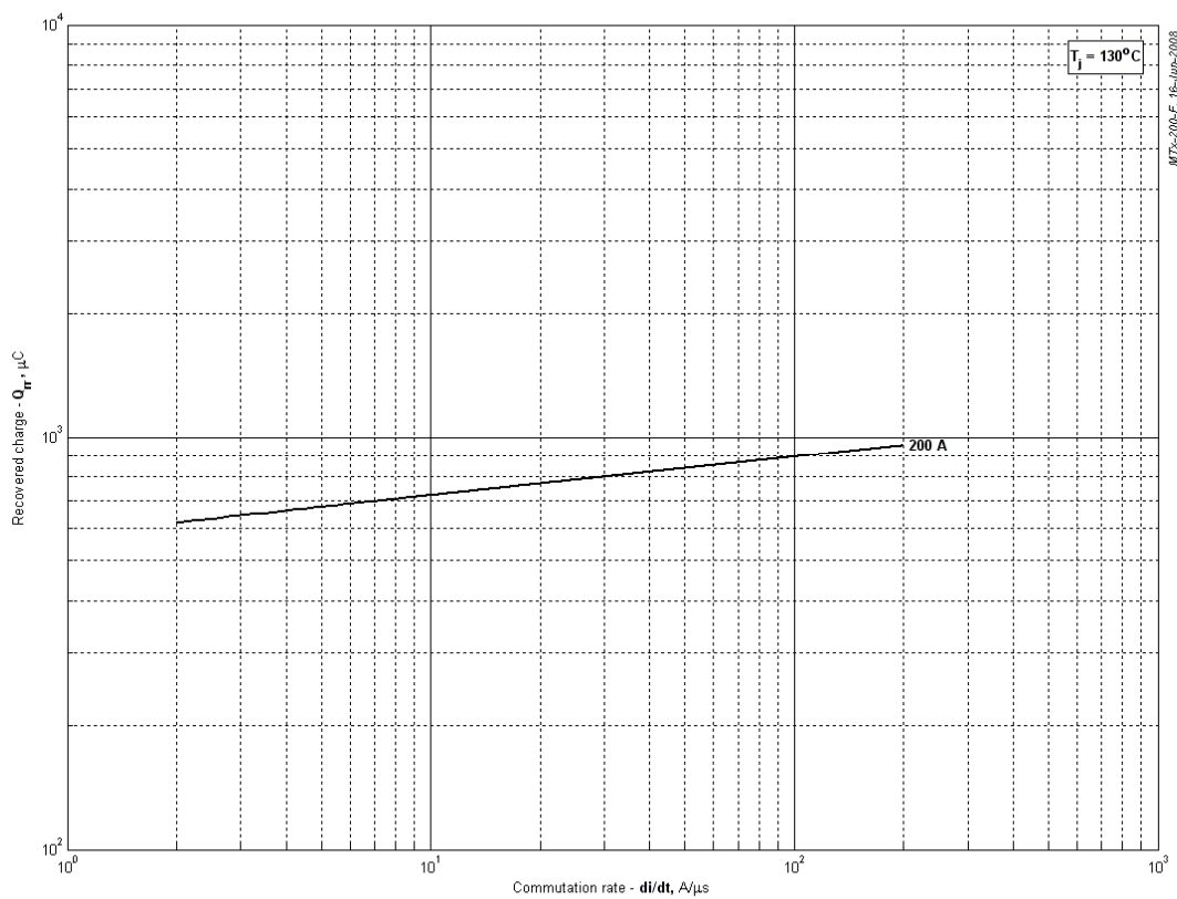
Fig 6 - Recovered charge, Q_{tr} (linear)
